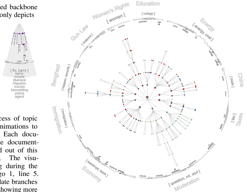
Fig. 5: IHTM result (with backbone; supervised SpecEx optimizations; no direct tree manipulations) for the second presidential debate between Romney and Obama in 2012 [17] in our topic-tree visualization.
